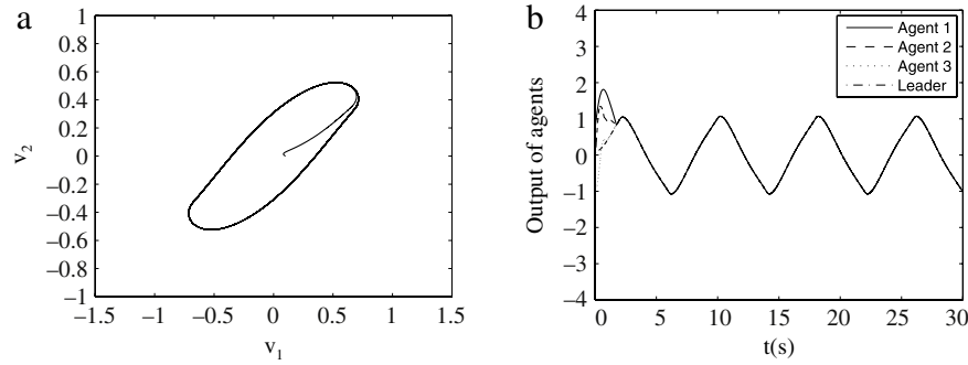
Fig. 2. Trajectory of the leader and performance of the control law.
